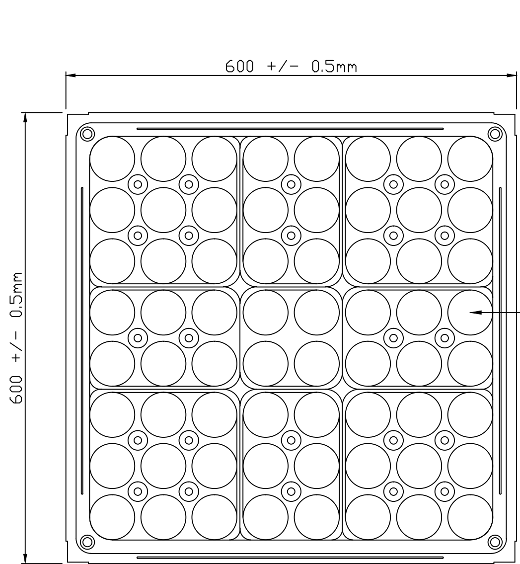
TYPICAL PANEL PLAN
