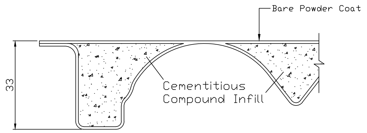
TYPICAL PANEL SECTION
